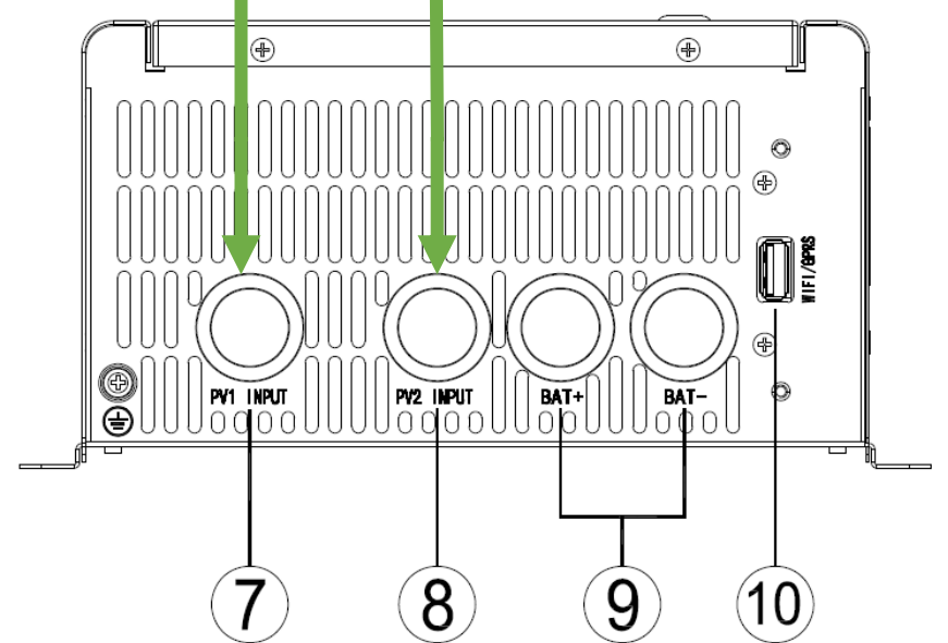
Wiring Diagram - Dual PV Array
